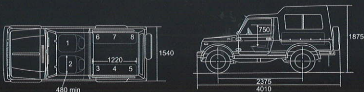
All Dimensions in mm. Shown Soft top Version.
