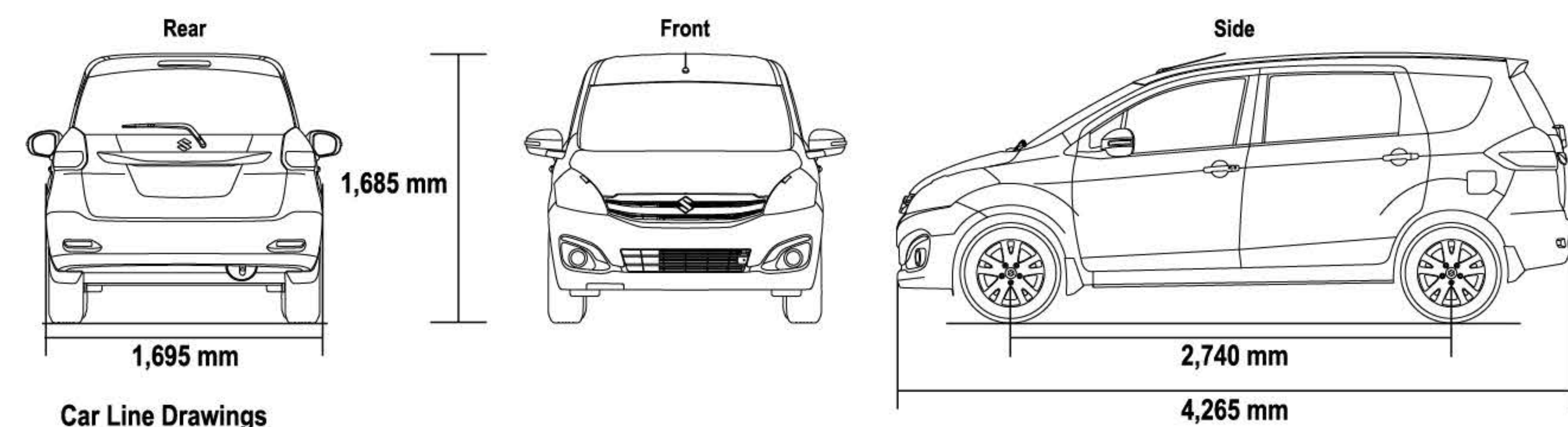
Car Line Drawings
